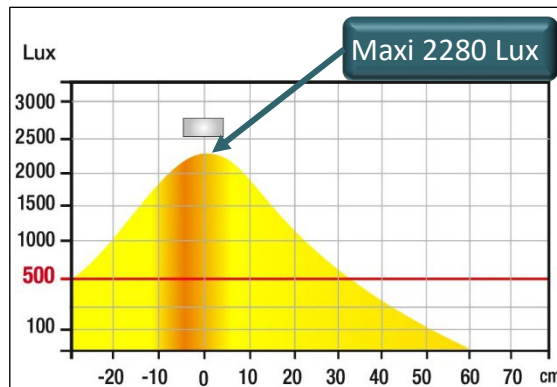
Measurement of Lux on the worktop in 35 cm profile view:
