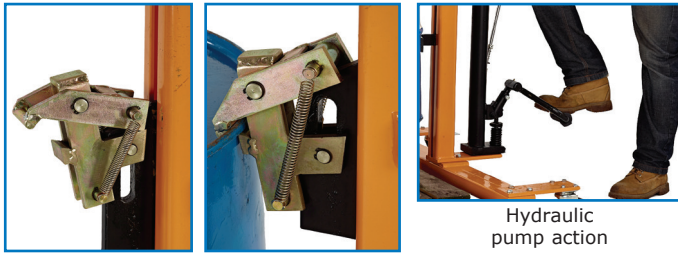
Drum locking mechanism
