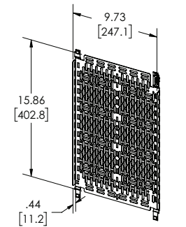
LEVER LOCK PANEL DETAIL
