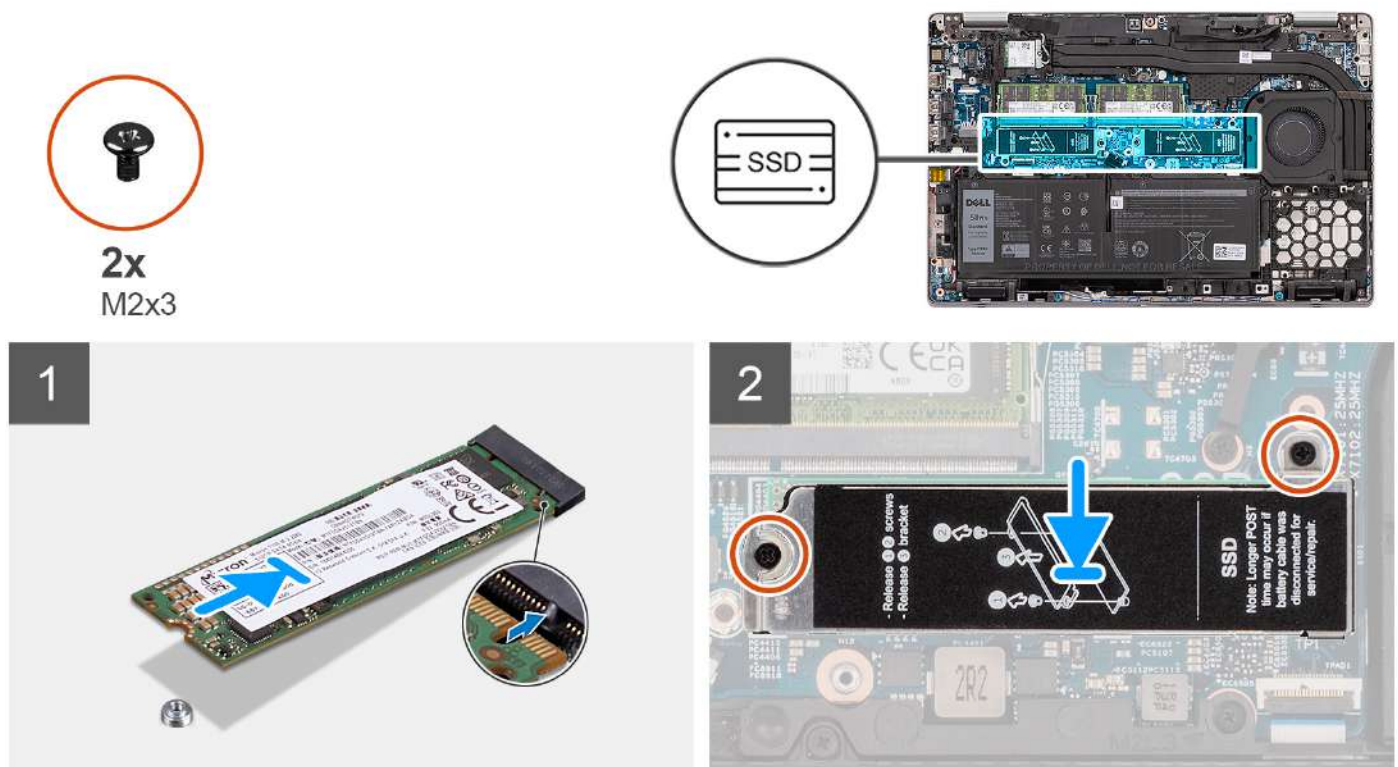
Figure 4. M.2 2280 solid-state drive with bracket
