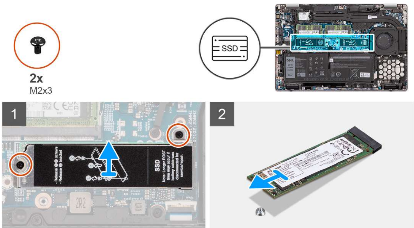
Figure 2. M.2 2280 solid-state drive with bracket
